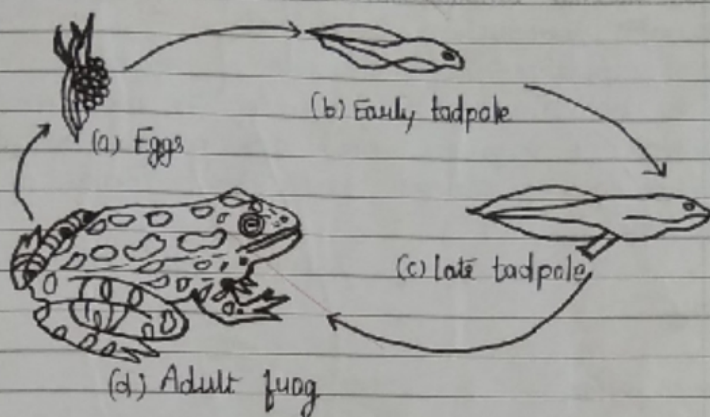
Fig 9.10: Life cycle of frog
