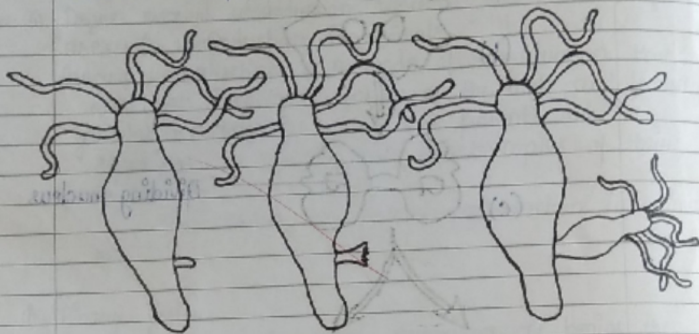
Fig. 9.11 : Budding in Hydra.
